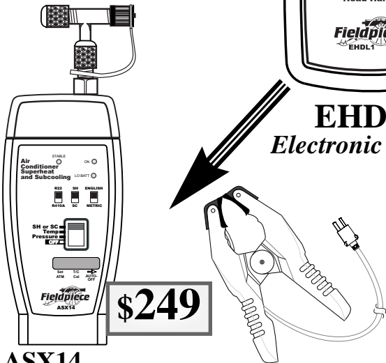
ASX14 Superheat and Subcooling (R22 & R10A) A/C Charging Kit w/ ATC1 Pipe Clamp (ATC1)
